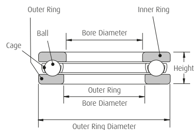
Single Direction Thrust Ball Bearing
