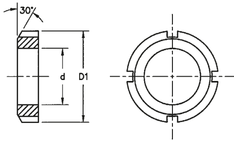
Inch Lock Nuts
