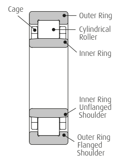
Cylindrical Roller Bearing (NU Style)
