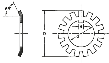
Inch Lock Washers
