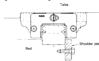
Recommended Torque for Rail Mounting Bolt (Case of Thermally Refined Bolt) unit: kgf · cm
